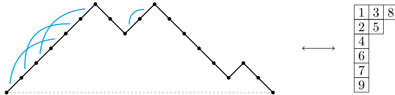
FIGURE 4.5. The cm-labeled Dyck path D and its corresponding SYT T_D .
