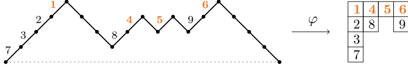
FIGURE 2.1. Example of the map \varphi , where the columns of the array on the right are the blocks of the resulting nonincreasing partition.
