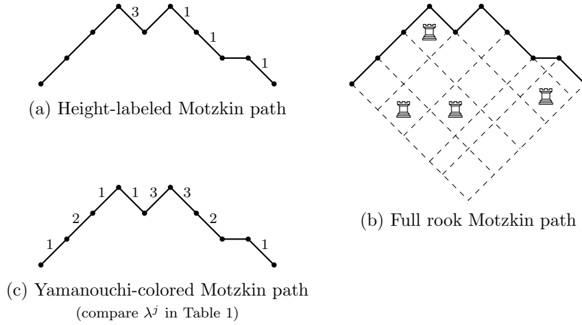
FIGURE 6.1. Motzkin paths corresponding to (1\ 6)(2\ 7)(3\ 4)(5\ 9)(8) .
